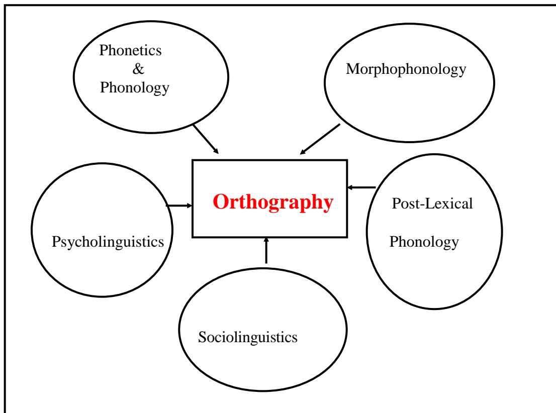
Diagram 1: Overall Architecture
